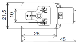
valve Connector type B 10mm
