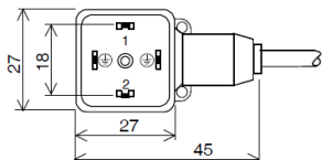
Valve Connector type A 18mm
